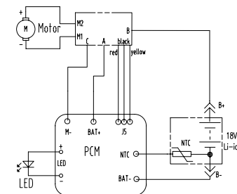
Electric circuit
