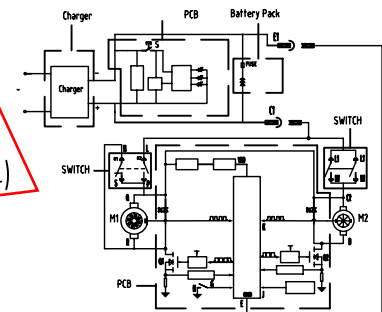
Electric Circuit
