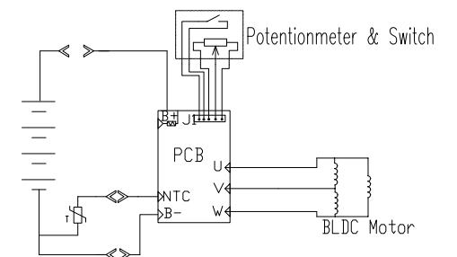
Electric Circuit
