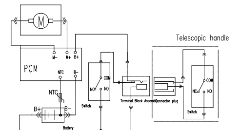
Electric circuit
