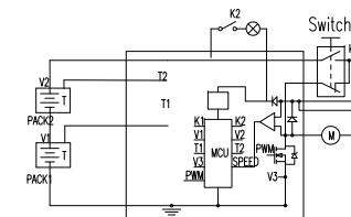
Electric circuit
