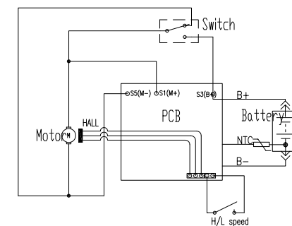
Electric circuit
