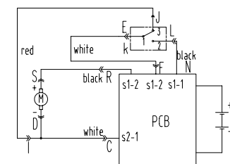
Electric circuit
