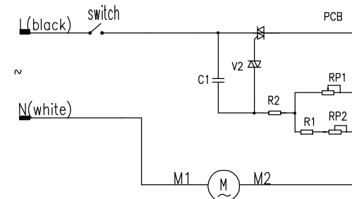
Electric Circuit
