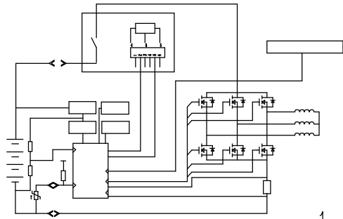
Electric circuit
