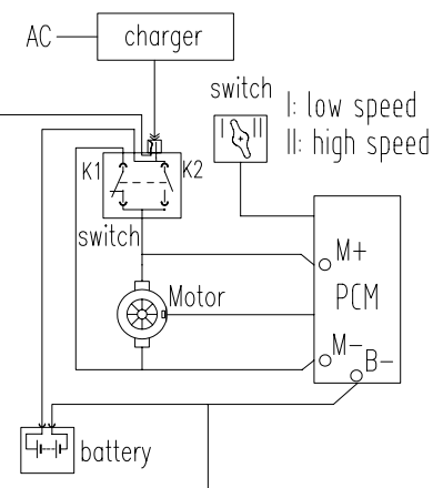
Electric circuit
