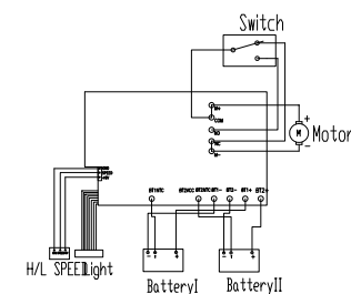
Electric circuit
