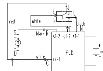
Electric circuit
